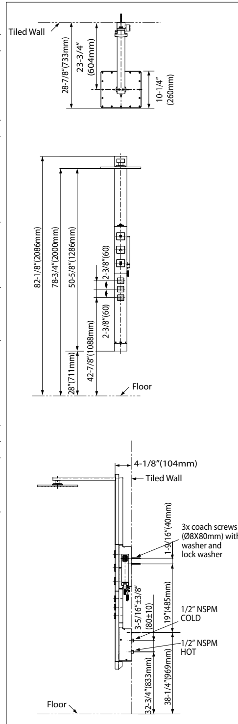
TS991A#CP - Neorest® Shower Tower
