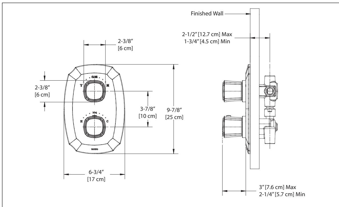
TS970D - Guinevere® Thermostatic Mixing Valve Trim with Dual Volume Control
