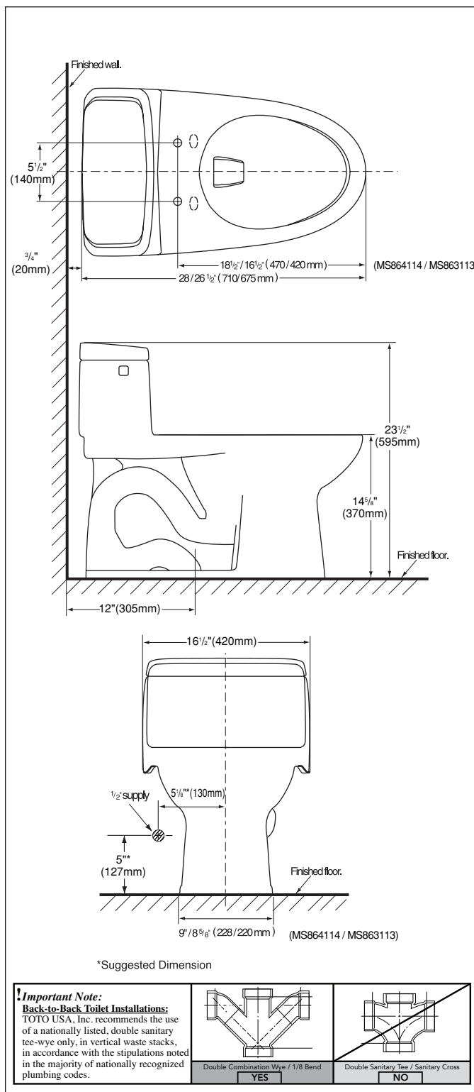
MS864114 / MS863113- Supreme Toilet with SoftClose Seat
