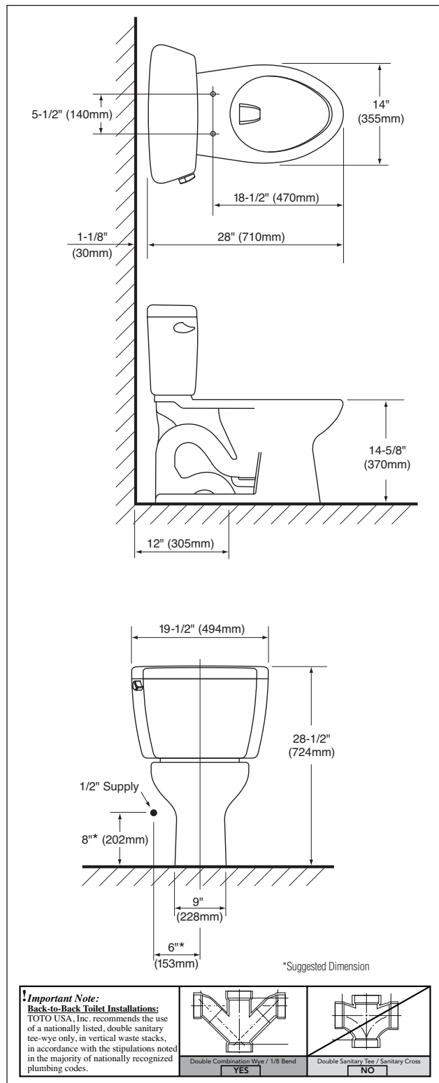
CST744S(G) - Drake Close Coupled Toilet
